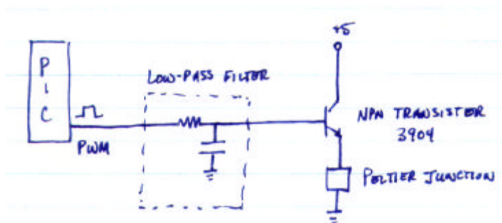
Figure 5.7 Circuit diagram of the "Heat" actuator
