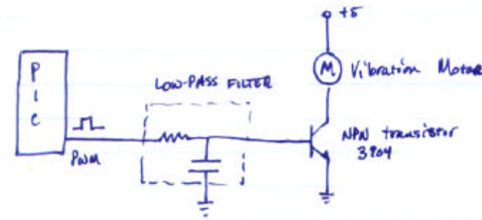
Figure 5.4 Circuit diagram for the "Shaker" actuator
