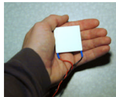
Figure 5.6 The front and side of a peltier junction
