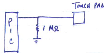
Figure 5.14 Circuit diagram for the touch sensor
